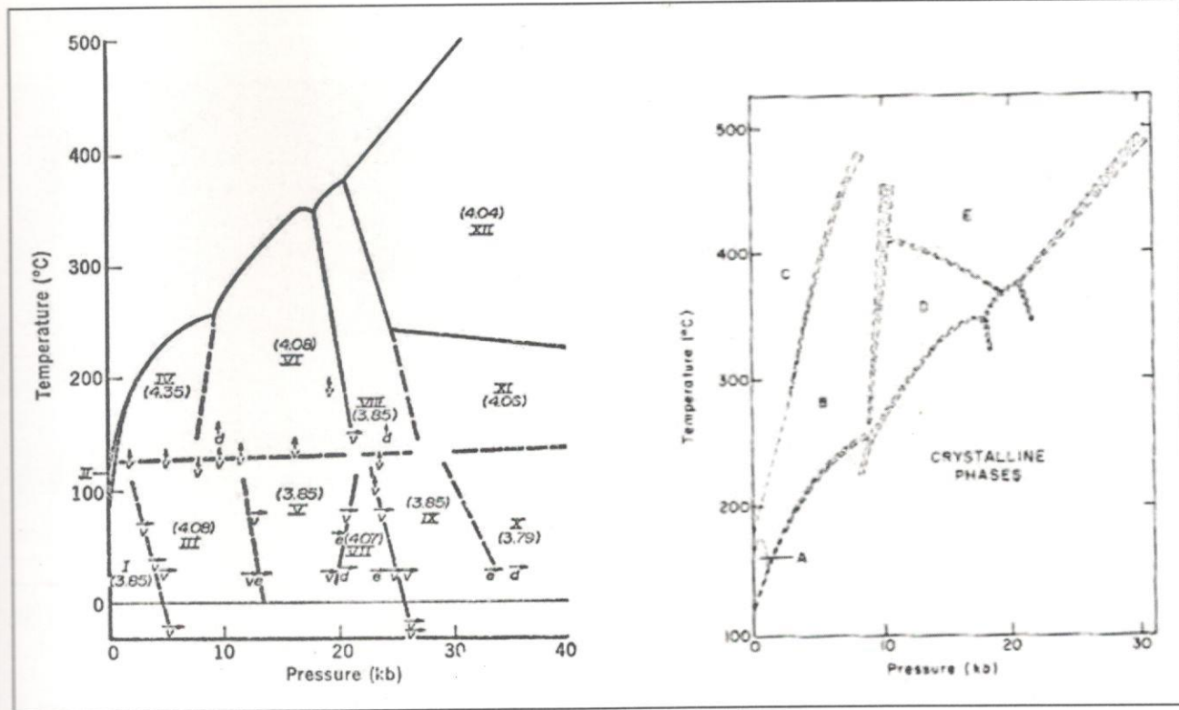
Fig. 4: P-T Phase Diagrams for sulfur (S). On the left is the sublucidus region showing the many crystalline structures. On the right is the liquid stable region showing at least 5 different liquid structures separated by a phase boundary.
