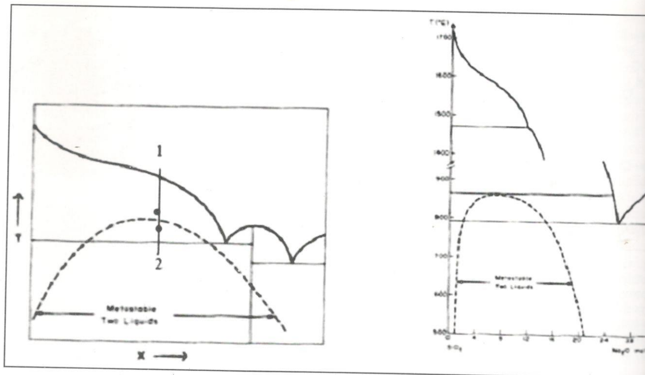
Fig. 3: The first presentation by Roy (1960) of the theoretical argument that the non-ideality of the liquidus (clearly shown its shape) indicated that the liquid phase itself was “heterogeneous” in structure, and could be induced to phase-separate a temperature region where it was metastable (left hand figure) [13]. Poraikoshits and Averjanov experimentally demonstrated exactly such an example in 1968 [14].
