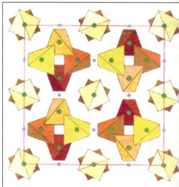
Fig. 10: Two of the "molecules" in inorganic materials illustrated in the garnet structure by the 4-coordinated (cornered) tetrahedral (colored yellow and orange in the middle of the four quadrants, and the 6-coordinated octahedra.
