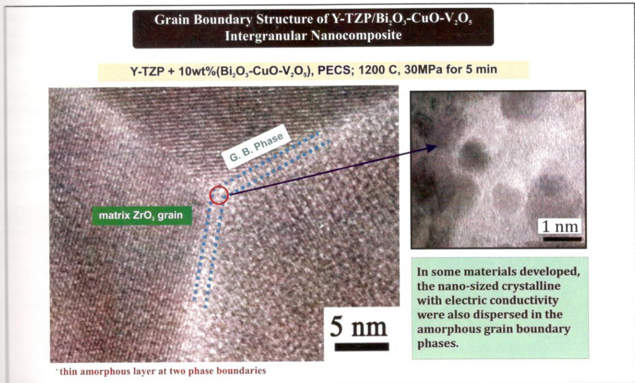
Fig. 12: Routine, typical TEM image of a complex crystalline composite at the nanometer level. Note the individual atoms all lined up in different arrangements, demanded by the structure. Specifically also note the intergranular matter, fuzzy and disordered. In the higher resolution blow up, one can see exactly what a typical, albeit multi-component, non-crystalline (like all liquids) area contains – disordered assemblages of different size (and composition, as revealed in the differences in contrast) typical of liquids. (From Niihara et al . [45]).
