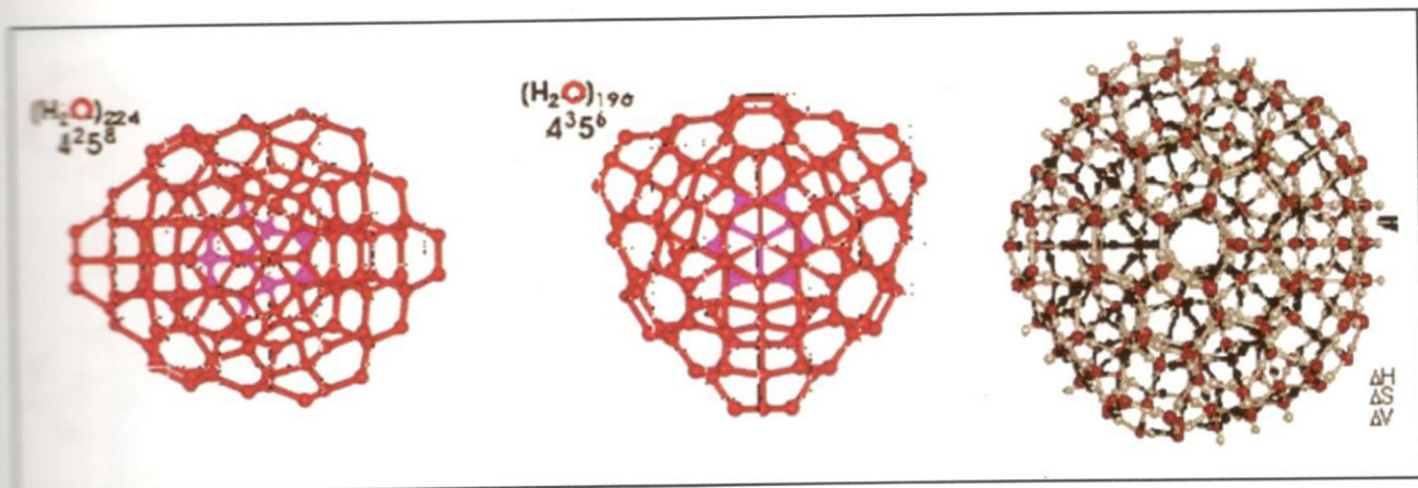
Fig. 9: This figure shows some of the larger polyhedra which are presumed to exist, largely on the calculation of likely structure of tetrahedrally bonded units. For refs. see Chaplin [38]. The relationship of the images of individual molecules, and how they are related to each other, in 3-D space, in liquid water, are rarely treated, the emphasis being on which units are present.
