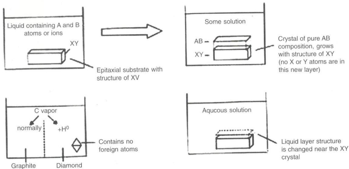
Fig. 14: A cartoon model of epitaxial transfer of structural information from one crystal to another, and to the liquid adjacent to the crystal without any transfer of composition. The graphite to diamond “determined” by the presence of H^{\circ} but no H is left in the diamond.
